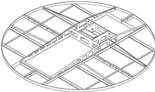
PITCHING MOUND FORMING SYSTEM Concrete for Synthetic Turf
