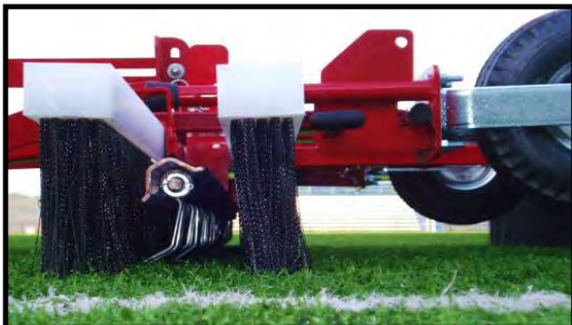
Spring Loaded Tines Setting
